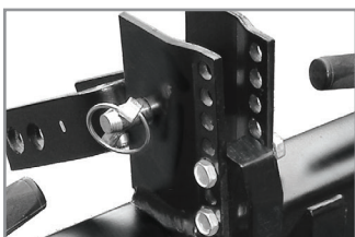
ADJUSTABLE TOP LINK BALL BRACKET
